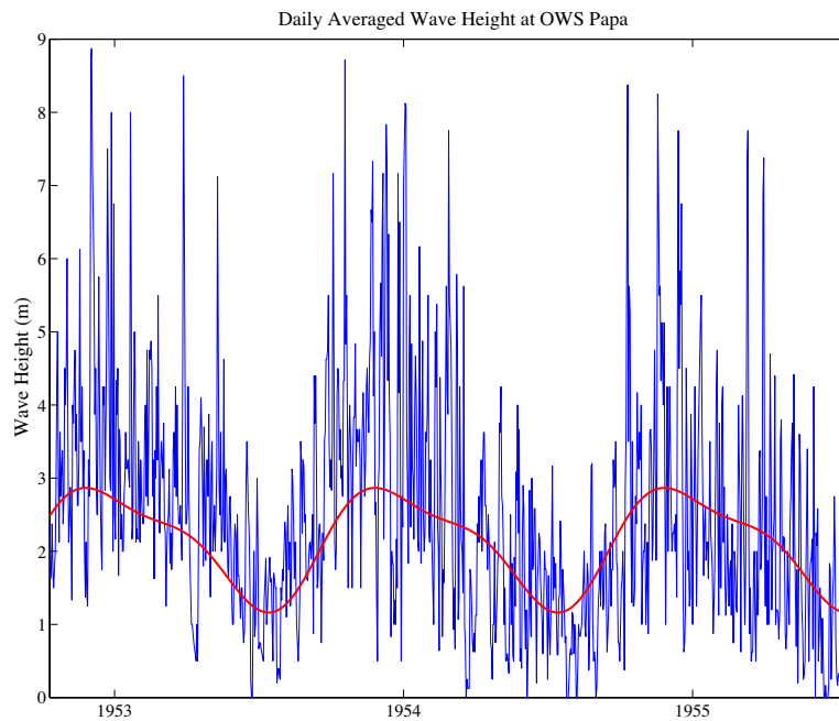
Figure 6. The modeled seasonal fluctuation in red aligns well with daily averaged wave height values.
