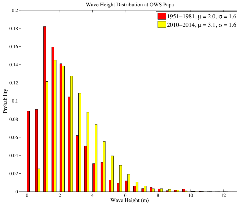
Figure 3. Statistical distribution of wave height at OSP. The mean ( \mu ) values of the historical wave height (red) and the modern wave height (significant wave height; yellow) indicate differences introduced by data collection methods. Historical measurements were collected visually, whereas a buoy that calculates significant wave height from a wave spectrum collects modern measurements. It should be noted that similar standard deviation values ( \sigma ) indicate that visual estimates were systematic and, therefore, remain useful to this analysis.
