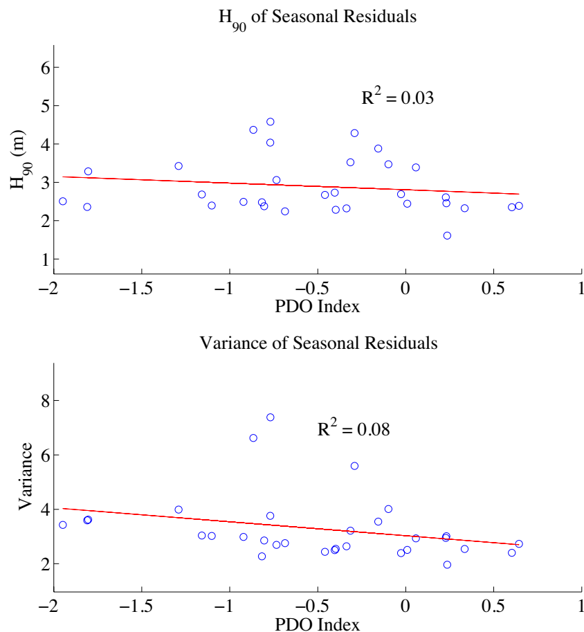
Figure 8. H_{90} and seasonal residual variance versus PDO index. In both cases, a weak dependence on PDO phase is demonstrated, though the dependence is stronger than observed in wind measurements.
