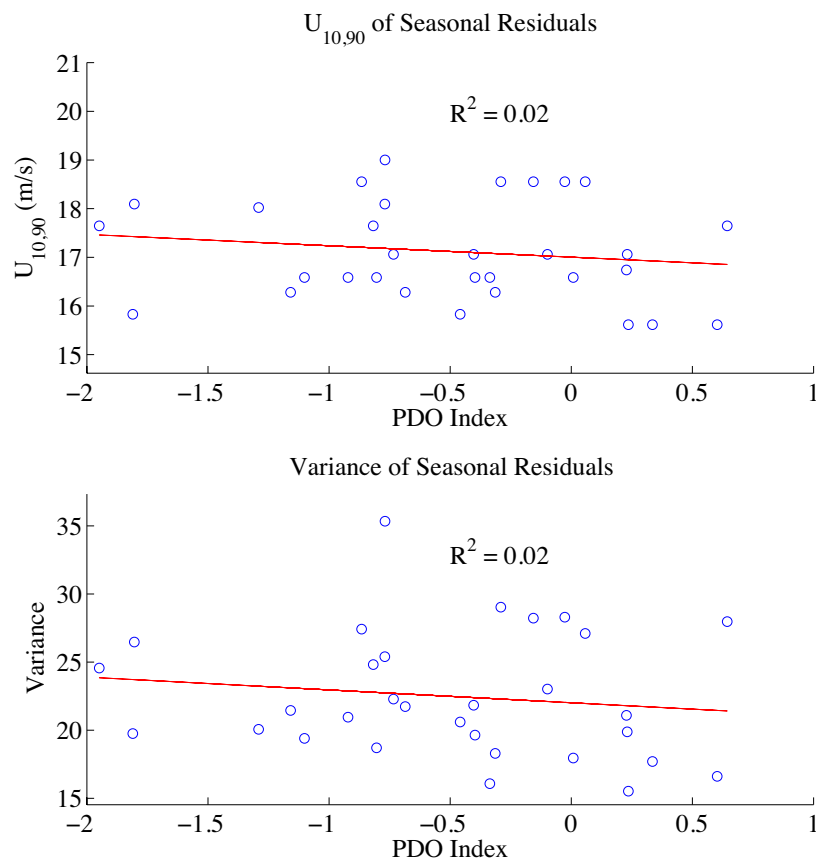
Figure 7. U_{10,90} and seasonal residual variance versus PDO index. In both cases, a weak dependence on PDO phase is demonstrated.
