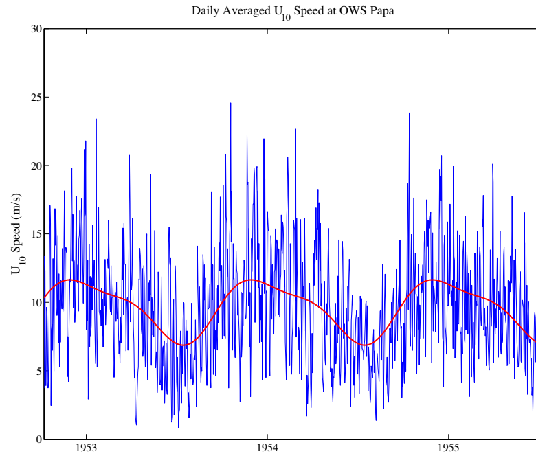
Figure 5. The modeled seasonal fluctuation in red aligns well with daily averaged U_{10} values.
