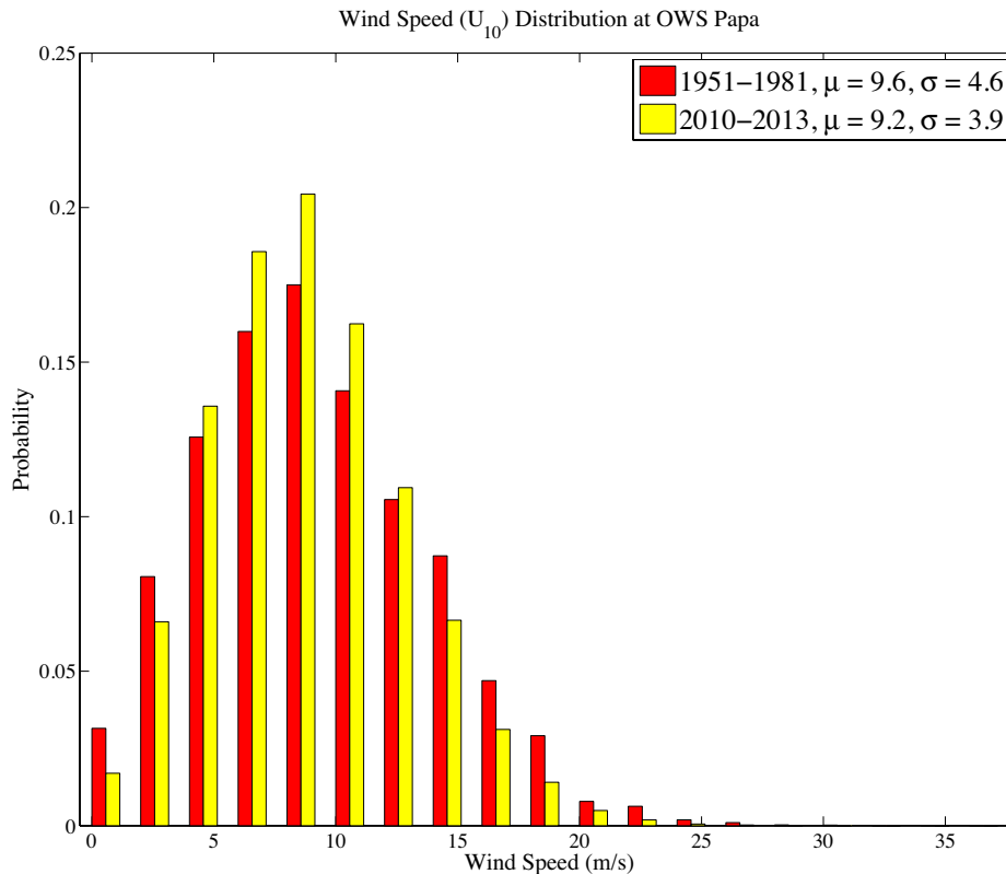
Figure 2. Statistical distribution of U_{10} speed at OSP. The statistical mean ( \mu ) and standard deviation ( \sigma ) show close agreement between the historical data (red) and the modern data (yellow).
