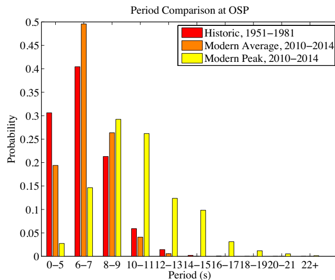
Figure 4. Historical and modern wave period values from OSP. The period of historical waves (red) agrees more strongly with the average period (orange) than the peak period (yellow) of modern waves.
