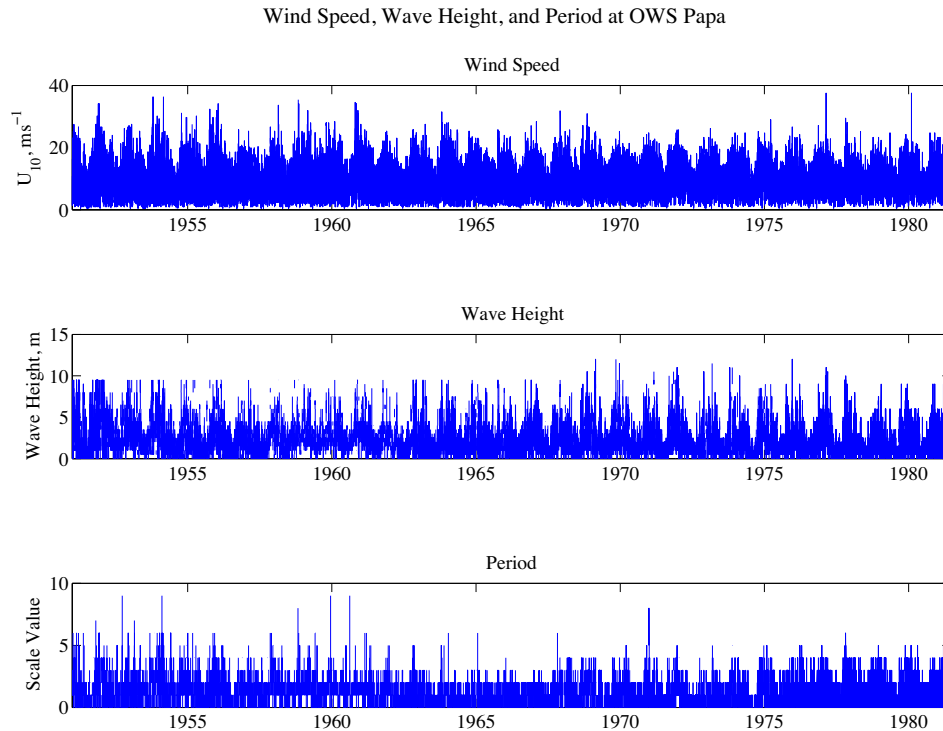
Figure 1. Full time series of wind speed, wave height, and wave period at OSP. Note: Period was reported using the following scale values: 0 (<5 s), 1 (6–7 s), 2 (8–9 s), 3 (10–11 s), 4 (12–13 s), 5 (14–15 s), 6 (16–17 s), 7 (18–19 s), 8 (20–21 s), 9 (>21 s).
